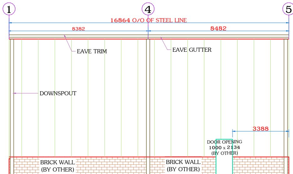
SIDE WALL SHEETING @ GRID-C
