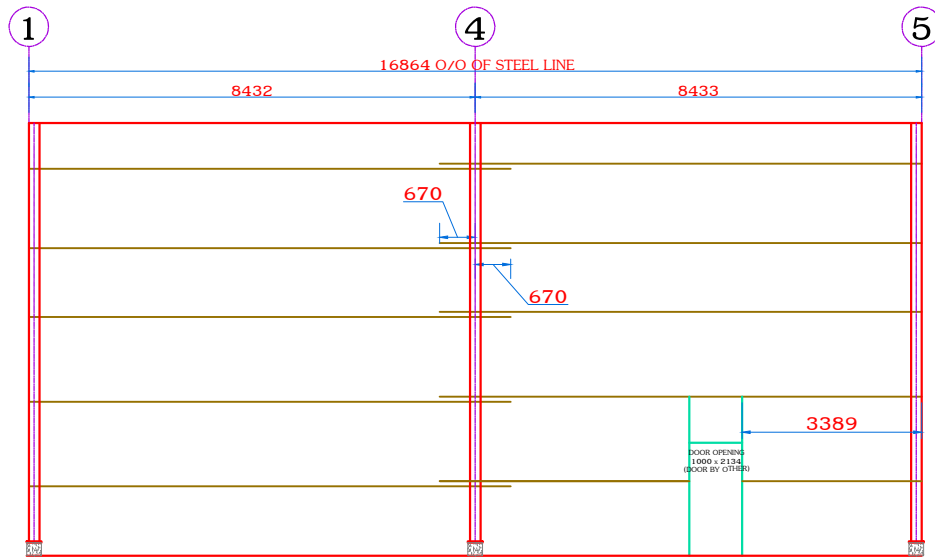
SIDE WALL FRAMING @ GRID-C
